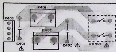
POWER SW PCB L6038A502D
