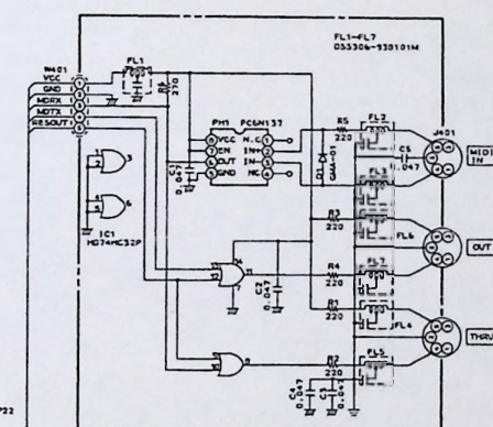
MIDI PCB L6028B504C
