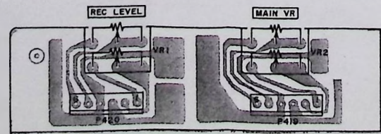
VR PCB L6028B504H(J1)
