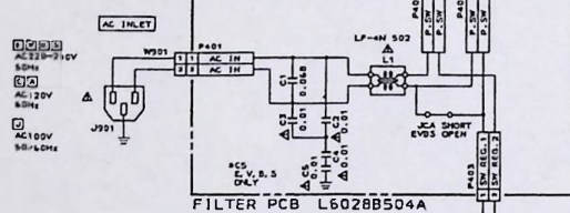
FILTER PCB L6028B504A
